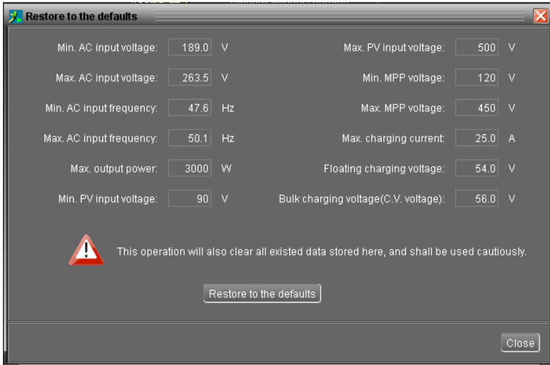
Diagram 4-12B (Off-Grid)
