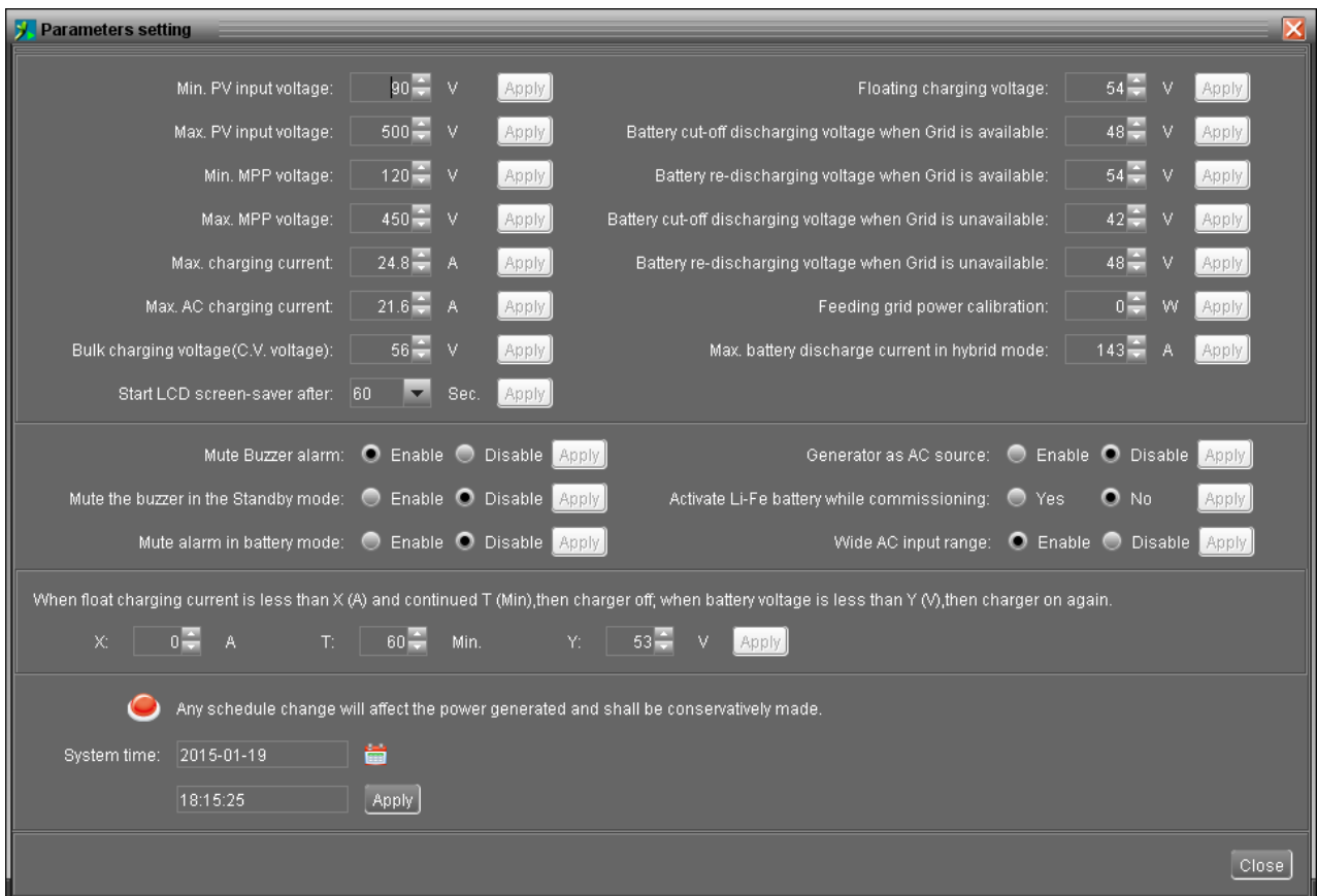
Diagram 4-11C (Off-Grid mode)
